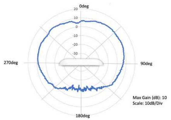
5 GHz Elevation
