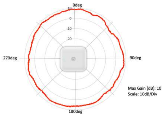
5 GHz Azimuth
