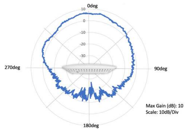
5 GHz Elevation
