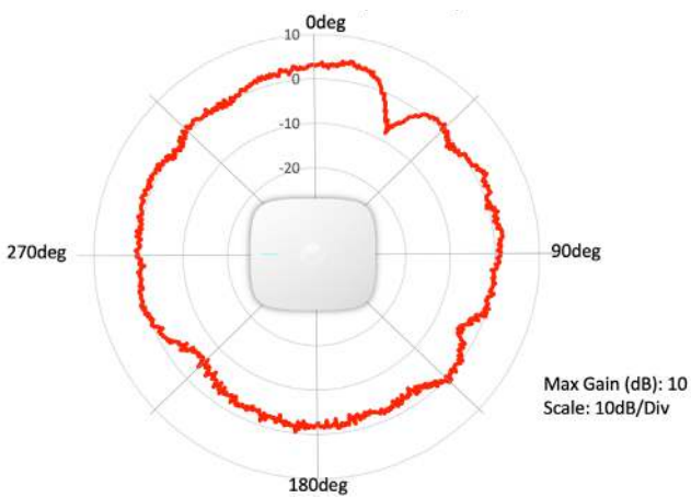
5 GHz Azimuth
